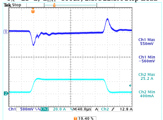
Pulsed-load Performance
