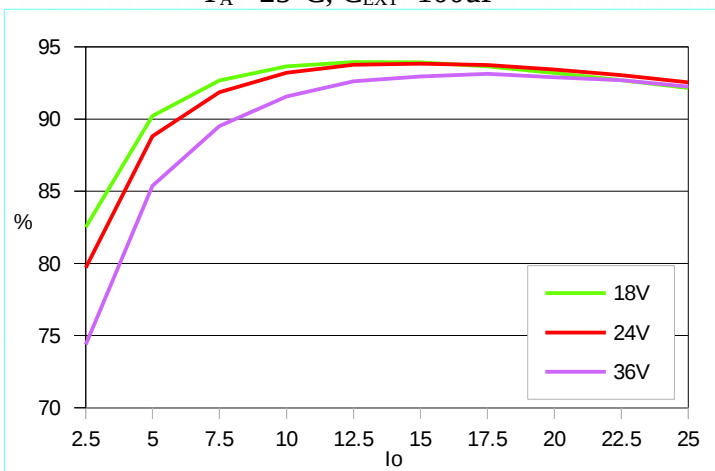
Conversion Efficiency
